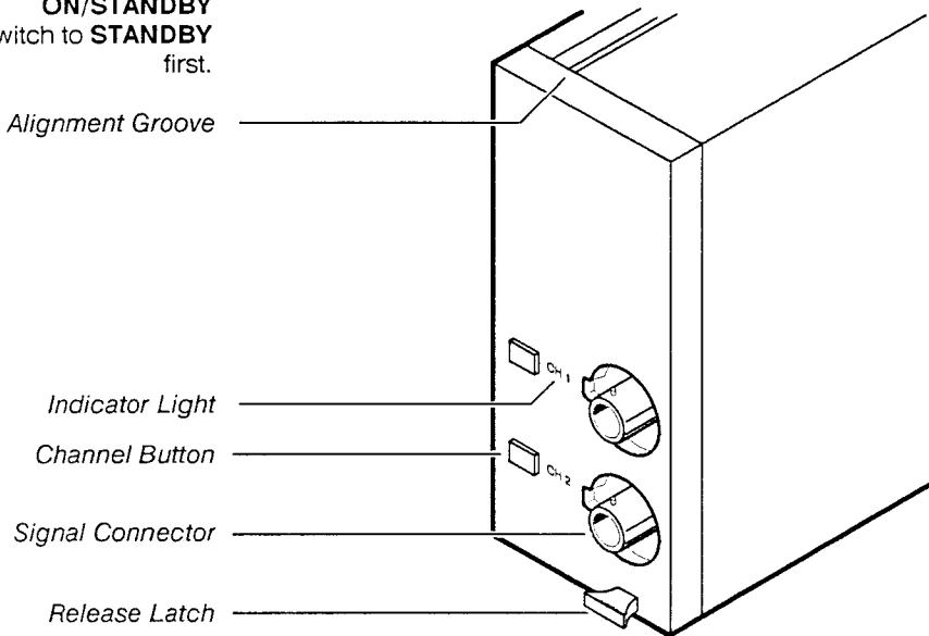
A Plug-in Amplifier
