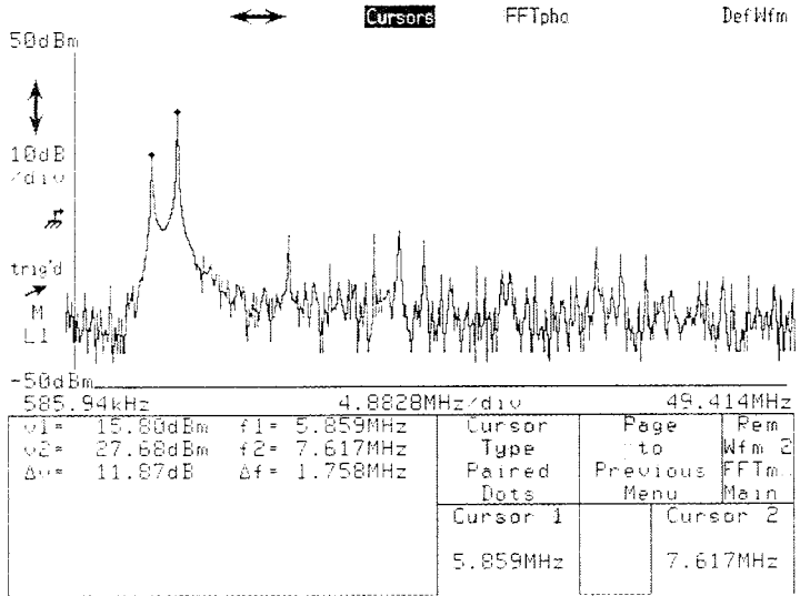
FFT Magnitude Displayed Using Rectangular Window
