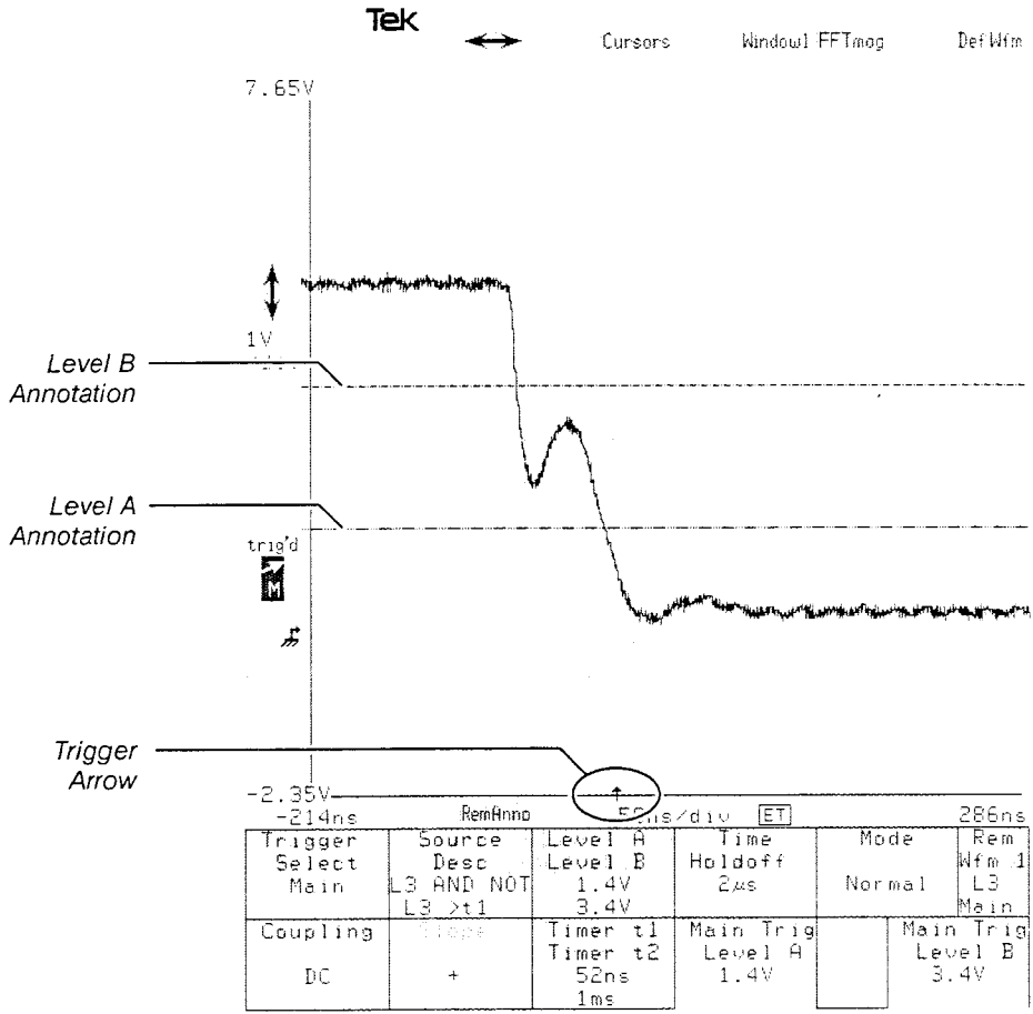
Example of Time Qualified Triggering
