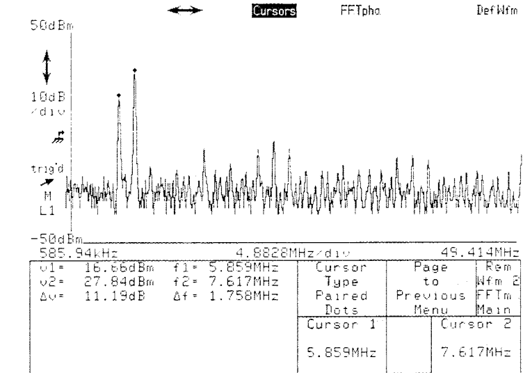
FFT Magnitude Displayed Using Hanning Window
